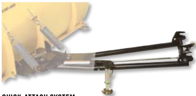
QUICK-ATTACH SYSTEM Available as an option to upgrade base Push Frame. The plough will be easy to install with this quick-attach system. Durable with a powder-coated rust-resistant finish. 715000731
